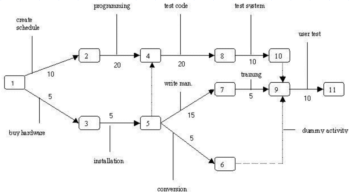
Fig. 1: PERT Chart
